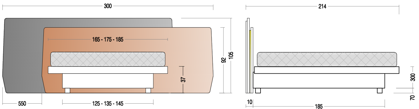
INTERSECO CONTENITORE INTERSECO WITH STORAGE
